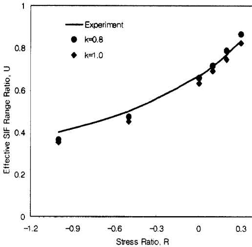
Fig. 3 Effective stress intensity factor range ratio, U , according to correction factors of element size calculated by reversed plastic zone size
